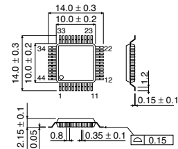
QFP44
